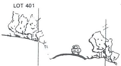
SOUTH COAST HIGHWAY SECTION 'A-A'
